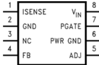
DGK Package 8-Pin VSSOP Top View
