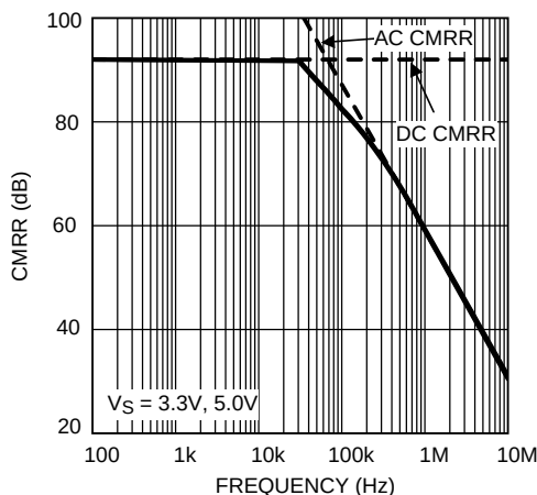
Figure 50. CMRR Curve
