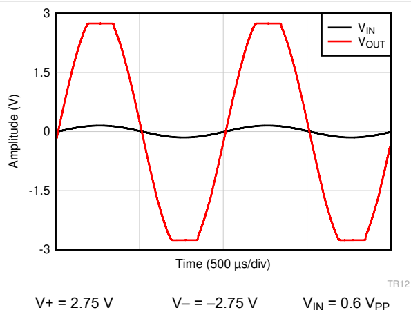
Figure 7-43. No Phase Reversal
