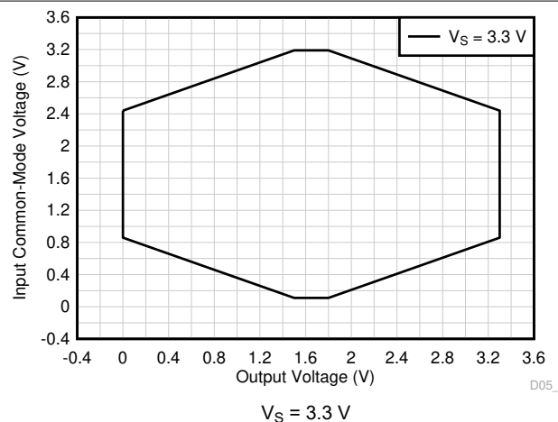
Figure 7-46. Input Common-Mode Voltage vs Output Voltage
