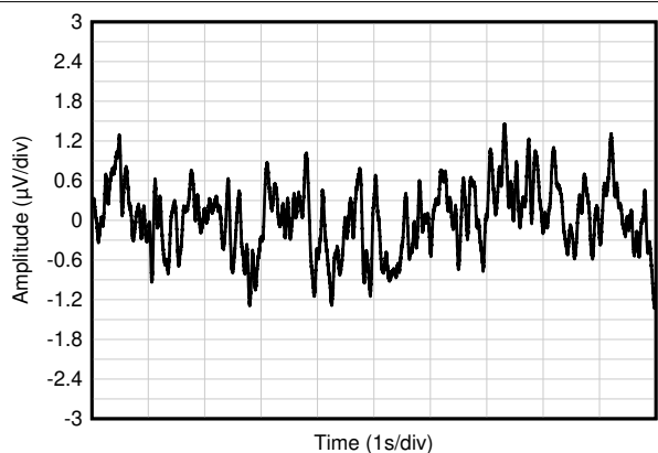
Figure 7-30. 0.1 Hz to 10 Hz Voltage Noise in Time Domain
