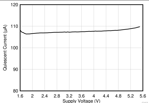
Figure 7-22. Quiescent Current vs Supply Voltage
