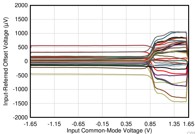
Figure 7-17. Input Referred Offset Voltage vs Input Common-Mode Voltage
