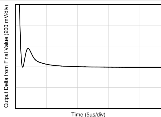
Figure 7-37. Large Signal Step Response
