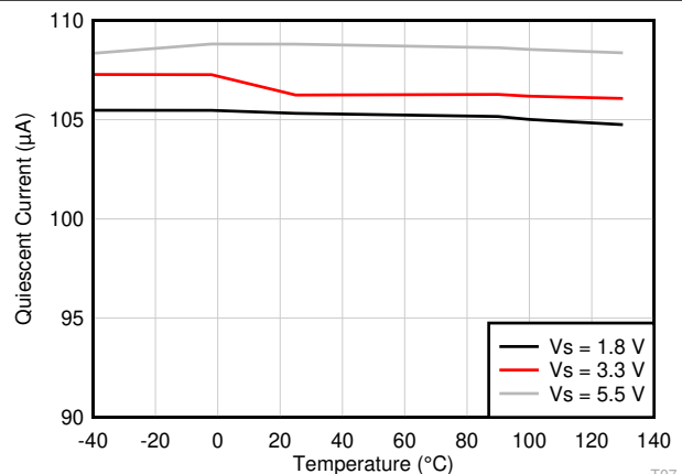
Figure 7-12. Quiescent Current vs Temperature
