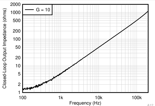
Figure 7-31. Closed-Loop Output Impedance vs Frequency
