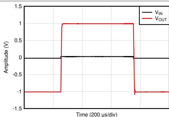
Figure 7-37. Large Signal Step Response
