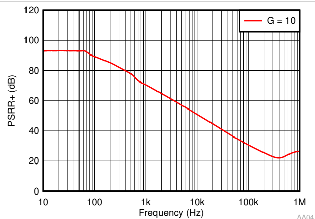
Figure 7-27. PSRR+ (Referred to Input) vs Frequency
