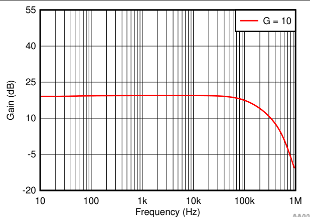
Figure 7-25. Closed-Loop Gain vs Frequency
