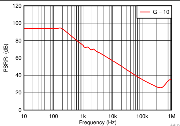
Figure 7-28. PSRR- (Referred to Input) vs Frequency
