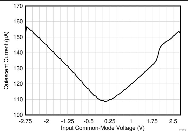
Figure 7-20. Quiescent Current vs Input Common-Mode Voltage
