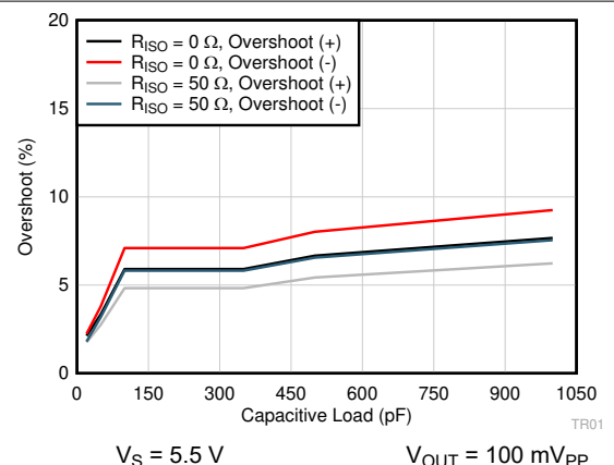
Figure 7-36. Small-Signal Overshoot vs Capacitive Load
