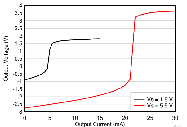
Figure 7-24. Output Voltage vs Output Current (Sinking)
