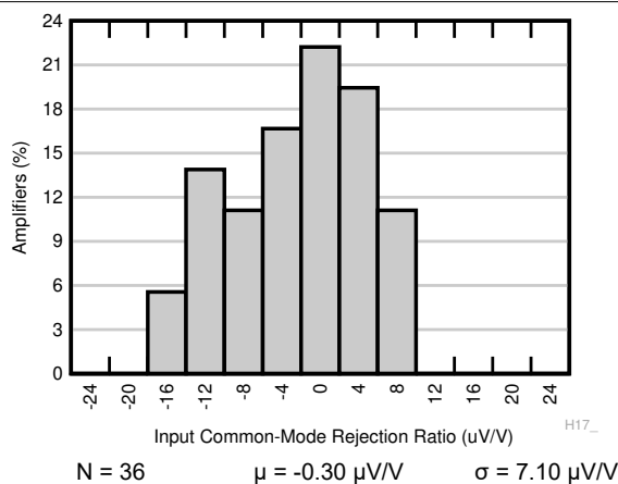
Figure 7-7. Typical Distribution of CMRR
