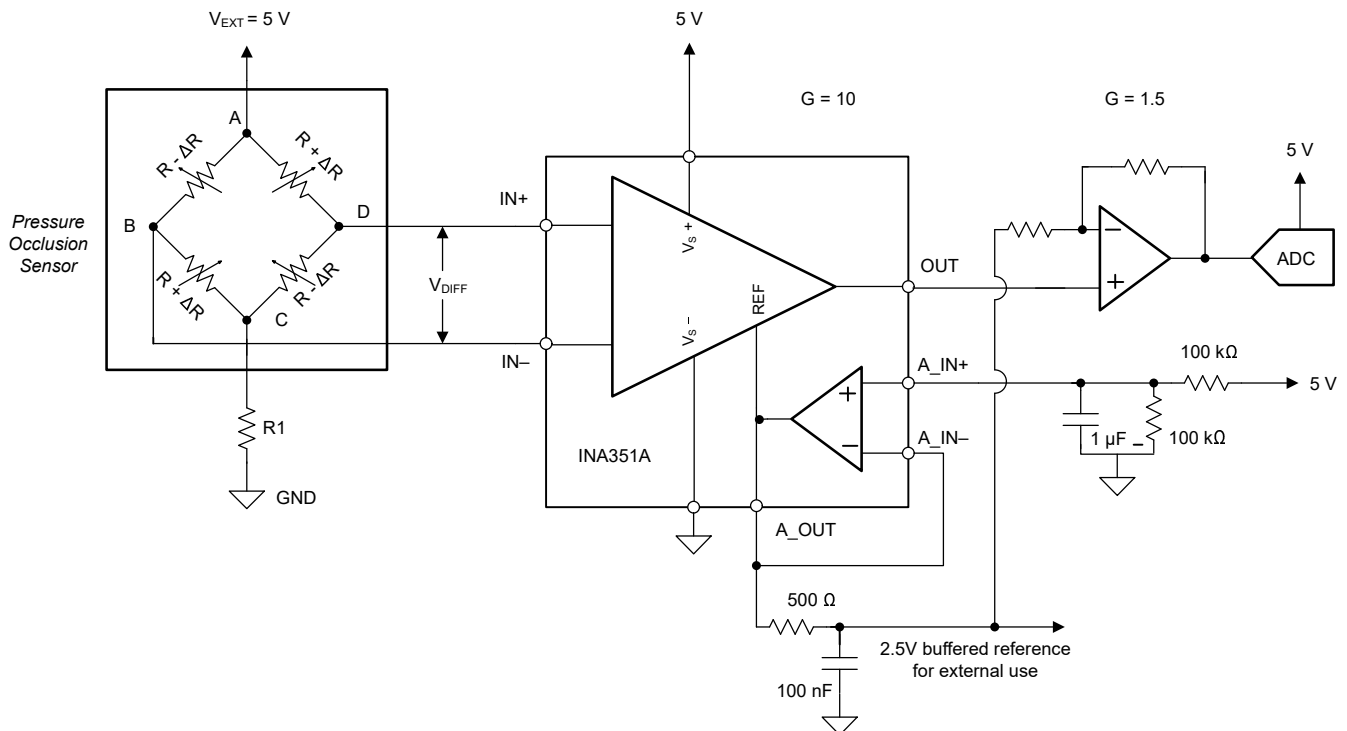
Figure 9-4. Resistive-Bridge Pressure Sensor
