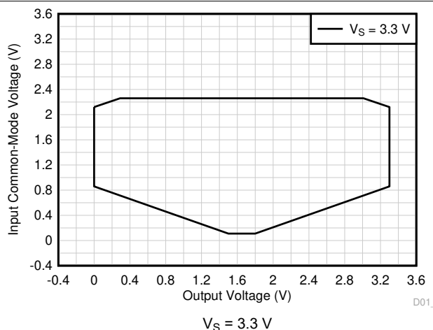
Figure 7-44. Input Common-Mode Voltage vs Output Voltage (High CMRR Region)
