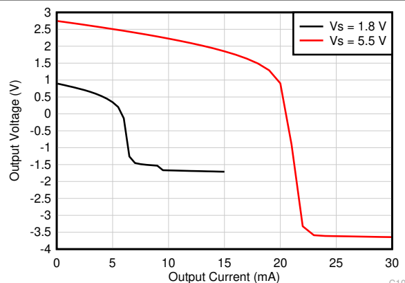
Figure 7-23. Output Voltage vs Output Current (Sourcing)
