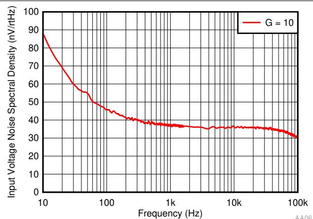
Figure 7-29. Input Referred Voltage Noise Spectral Density
