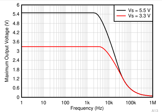
Figure 7-32. Maximum Output Voltage vs Frequency
