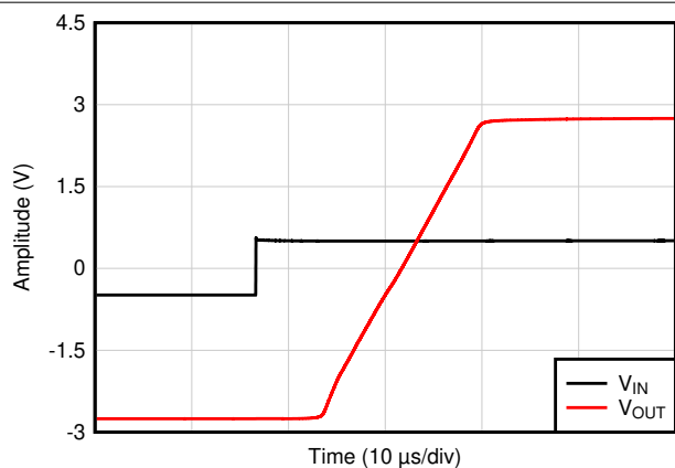
Figure 7-39. Large Signal Settling Time (Rising Edge)
