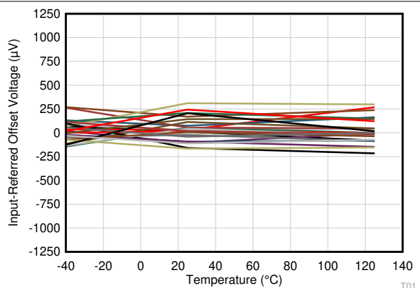
Figure 7-9. Input Referred Offset Voltage vs Temperature
