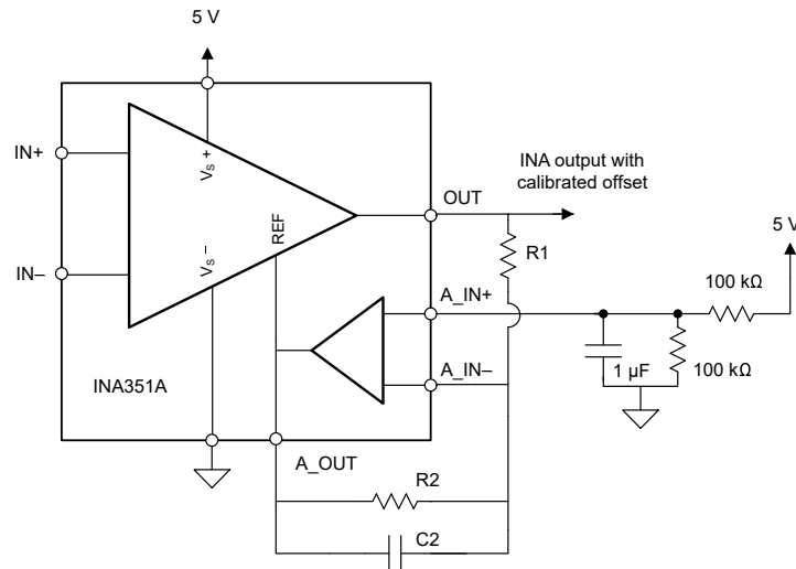
Figure 9-2. INA351A in Servo-Loop Calibration Configuration
