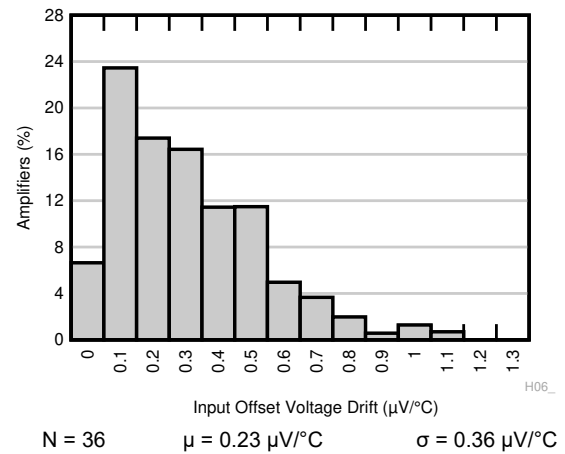
Figure 7-2. Typical Distribution of Input Referred Offset Drift
