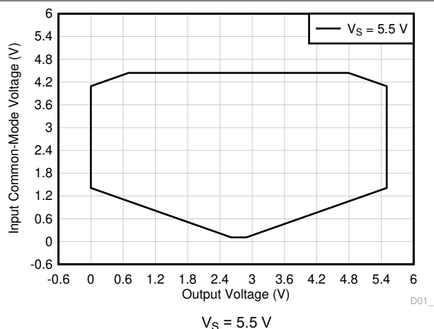
Figure 7-45. Input Common-Mode Voltage vs Output Voltage (High CMRR Region)
