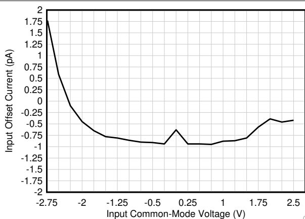
Figure 7-19. Input Offset Current vs Input Common-Mode Voltage
