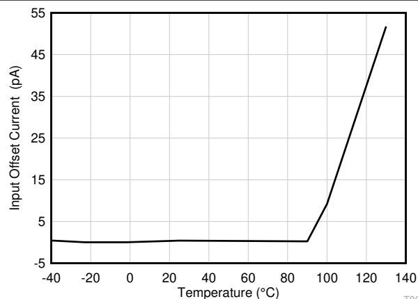
Figure 7-11. Input Offset Current vs Temperature
