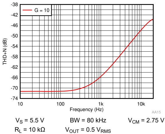
Figure 7-33. THD + N Frequency
