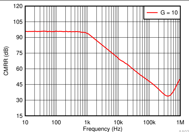
Figure 7-26. CMRR (Referred to Input) vs Frequency
