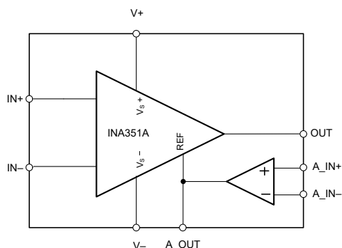
Simplified Internal Schematic
