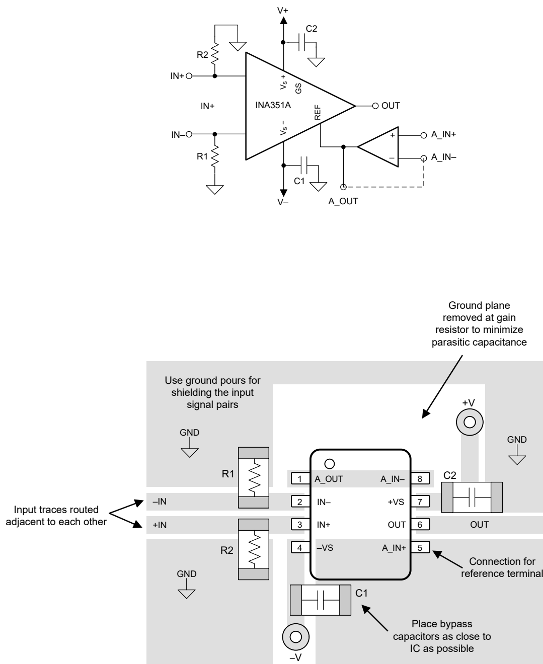
Figure 9-7. Example Schematic and Associated PCB Layout
