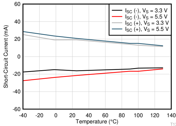
Figure 7-13. Short Circuit Current vs Temperature
