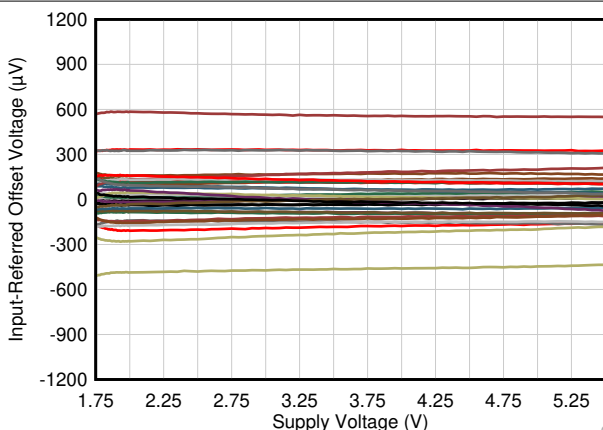
Figure 7-21. Input Referred Offset Voltage vs Supply Voltage
