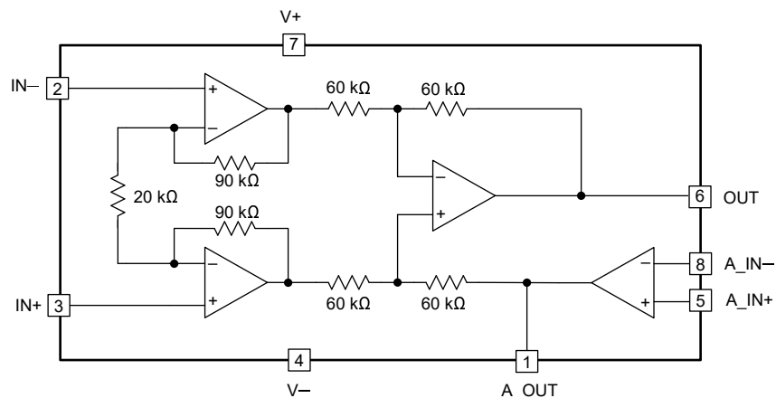
Figure 8-1. Simplified Internal Schematic
