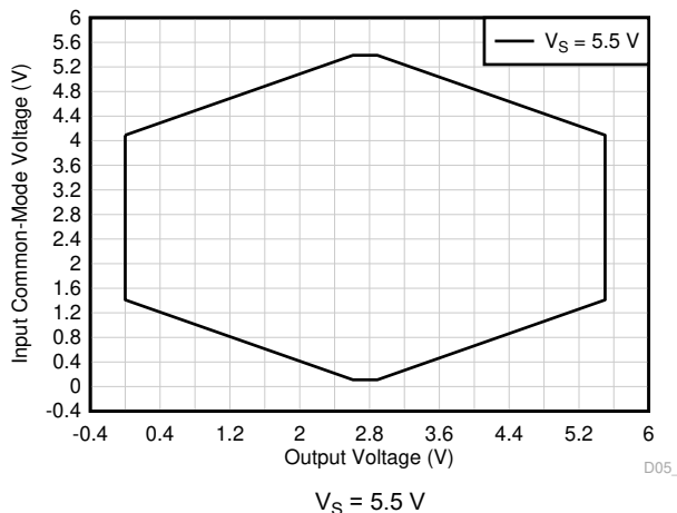
Figure 7-47. Input Common-Mode Voltage vs Output Voltage
