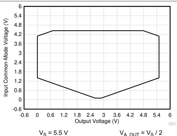
Figure 8-2. Input Common-Mode Voltage vs Output Voltage (High CMRR Region)
