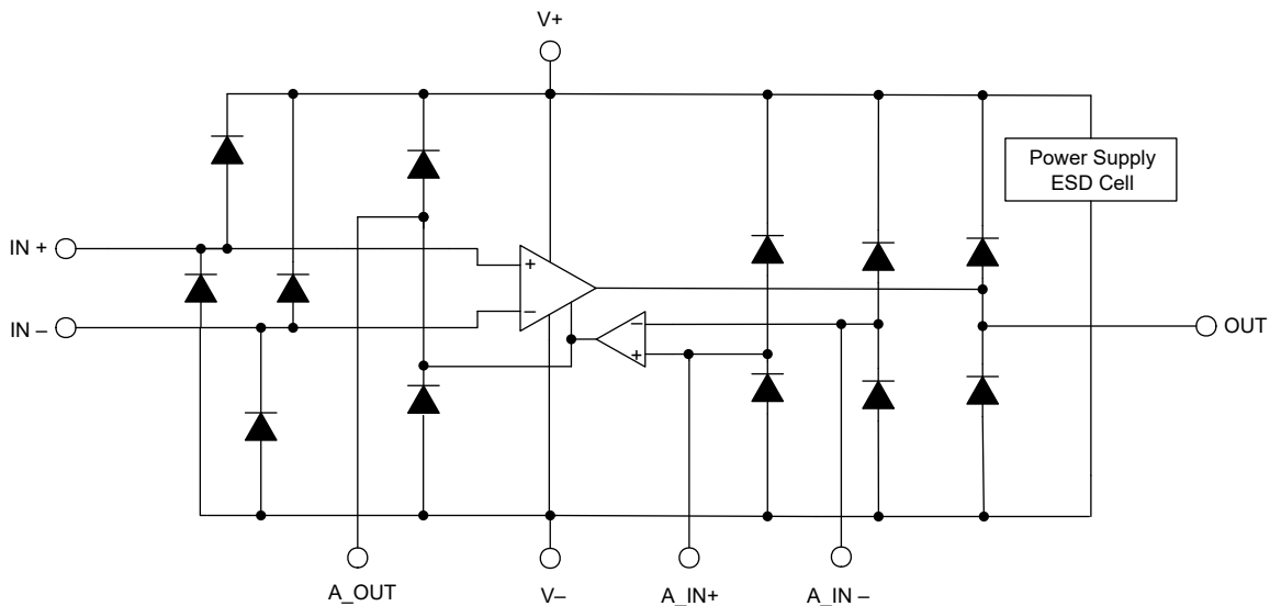
Figure 8-6. Equivalent Internal ESD Circuitry
