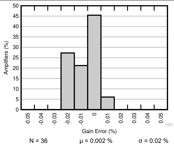
Figure 7-8. Typical Distribution of Gain Error
