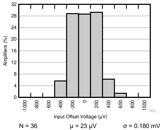
Figure 7-1. Typical Distribution of Input Referred Offset Voltage
