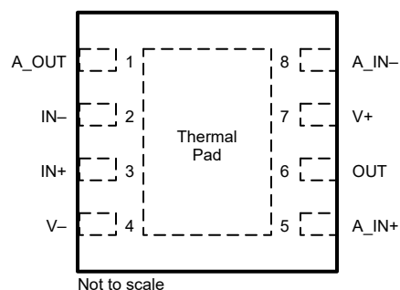
Figure 6-1. DSG Package, 8-Pin WSON With Exposed Thermal Pad (Top View)
