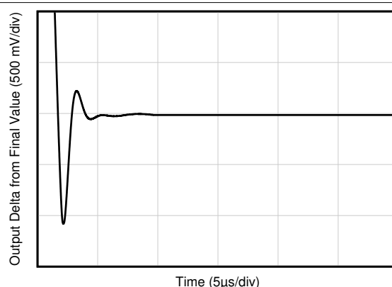
Figure 7-38. Large Signal Settling Time (Falling Edge)
