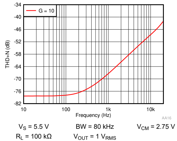
Figure 7-34. THD + N Frequency
