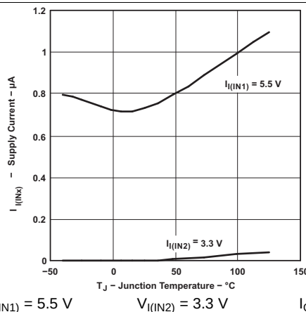
Figure 12. Supply Current vs Junction Temperature (Device Disabled)
