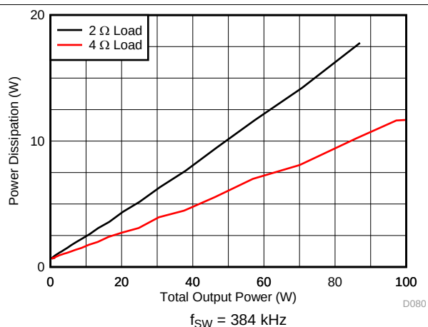
Figure 29. Power Dissipation vs Total Output Power
