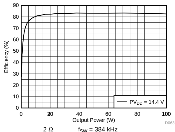
Figure 14. PVDD Power Efficiency vs Total Output Power
