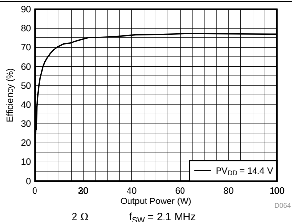
Figure 15. PVDD Power Efficiency vs Total Output Power
