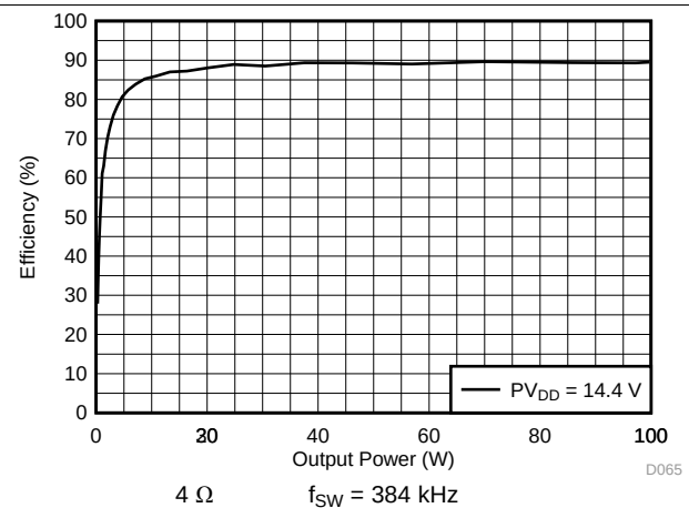
Figure 12. PVDD Power Efficiency vs Total Output Power
