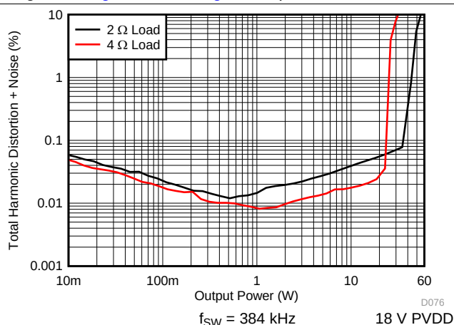
Figure 25. PBTL THD+N vs Power
