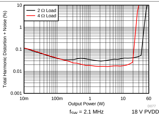
Figure 26. PBTL THD+N vs Power
