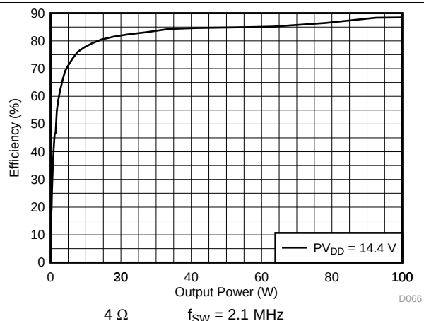
Figure 13. PVDD Power Efficiency vs Total Output Power
