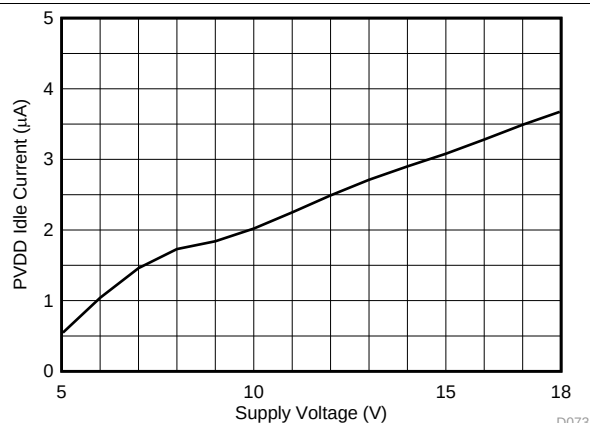
Figure 16. PVDD Idle Current vs Voltage
