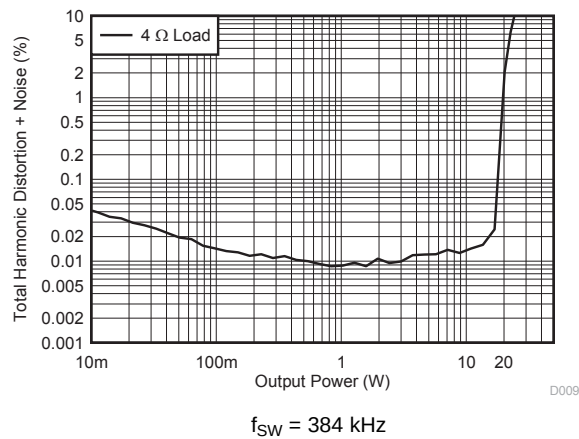
Figure 7. THD+N vs Power
