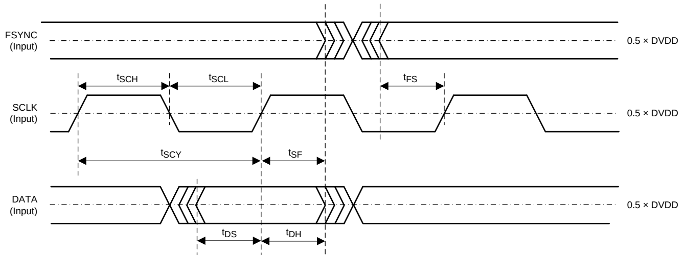
Figure 32. Serial Audio Timing
