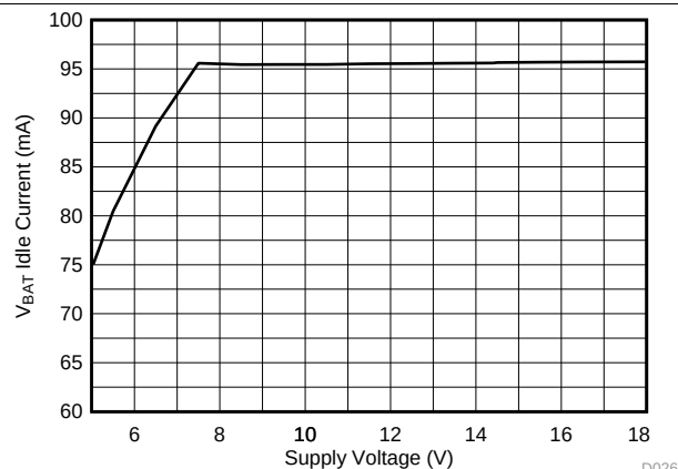
Figure 17. VBAT Idle Current vs Voltage
