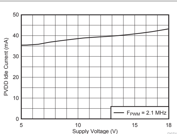
Figure 16. PVDD Idle Current vs Voltage
