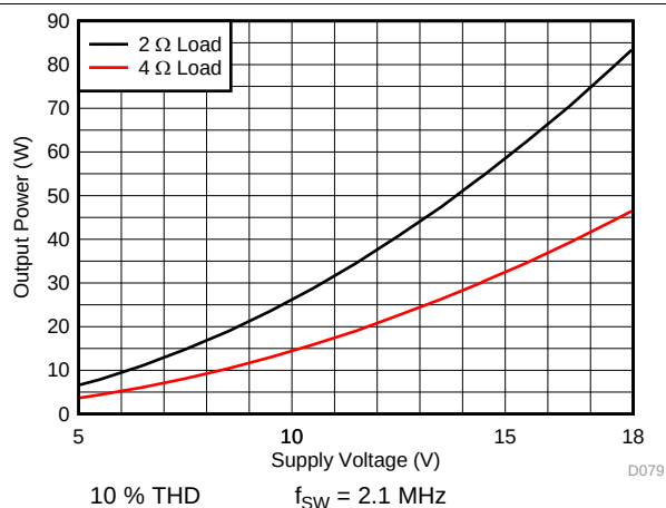
Figure 28. PBTL Output Power vs Voltage
