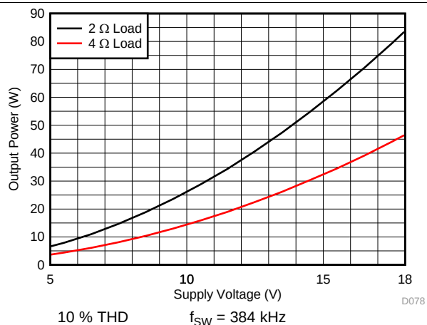
Figure 27. PBTL Output Power vs Voltage
