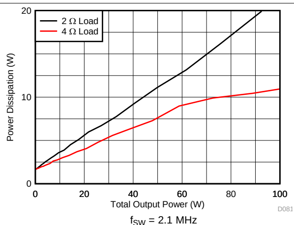
Figure 30. Power Dissipation vs Total Output Power
