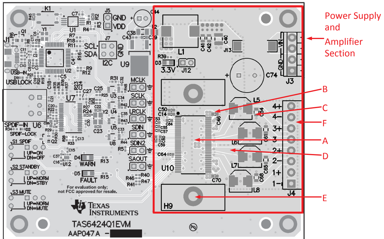
Figure 85. EVM Layout
