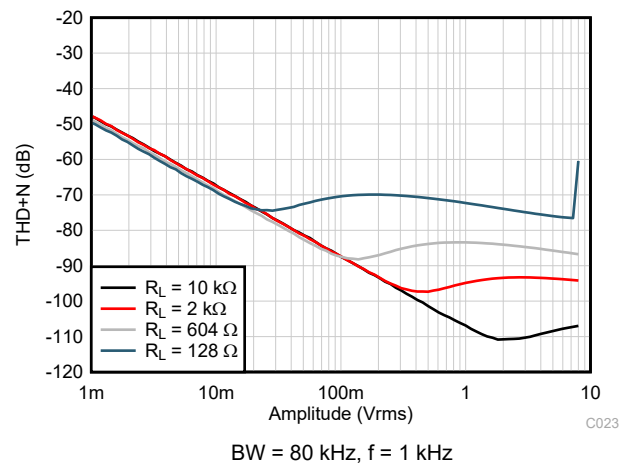
Figure 5-22. THD+N vs Output Amplitude
