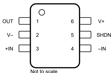
Figure 4-3. TLV9151S-Q1 DBV Package, 6-Pin SOT-23 (Top View)
