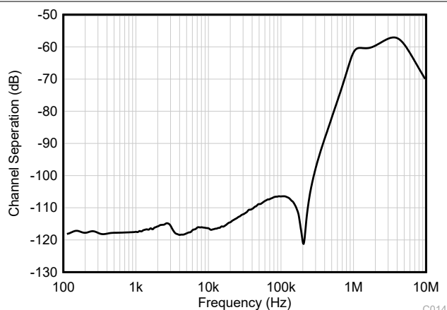
Figure 5-40. Channel Separation vs Frequency
