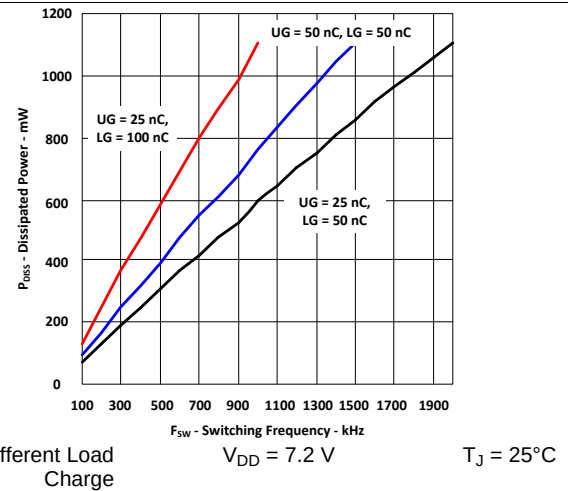
Figure 15. Driver Dissipated Power vs Switching Frequency
