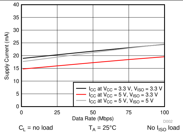
Figure 12. Supply Current vs Data Rate
