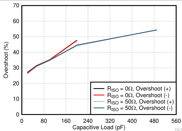
Figure 6-26. Small-Signal Overshoot vs Capacitive Load 20-mV pp Output Step, G = -1
