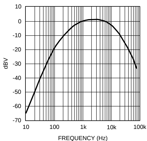
Figure 35. A-Weighted Filter
