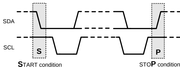
Figure 24. I²C Start Stop Conditions
