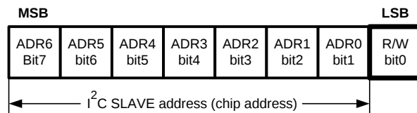
Figure 25. I²C Chip Address
