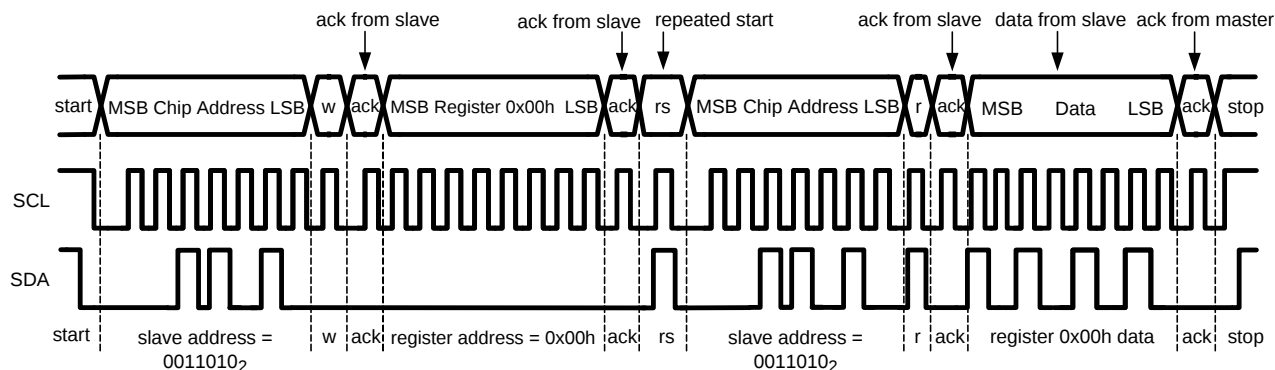
Figure 27. Example I²C Read Cycle
