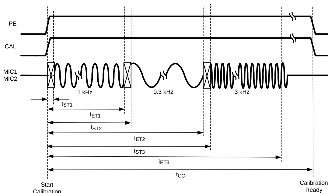
Figure 31. Calibration Timing
