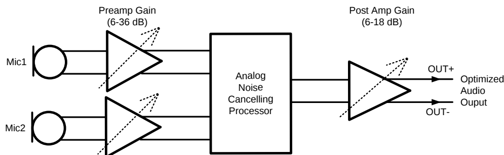
Figure 21. Simplified Block Diagram of the LMV1089
