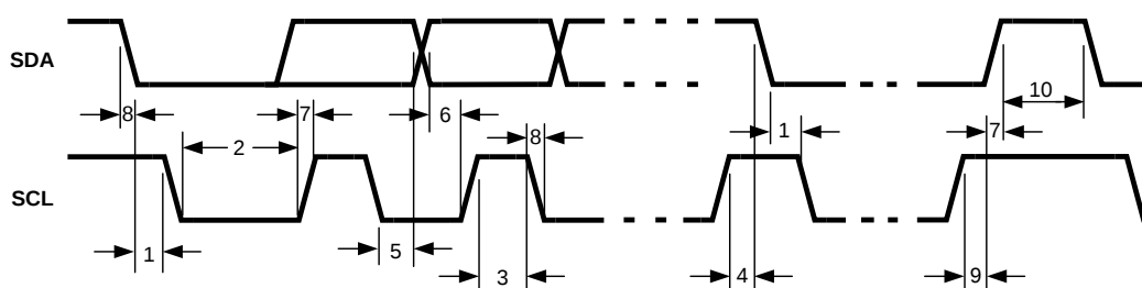
Figure 28. I²C Timing Diagram
