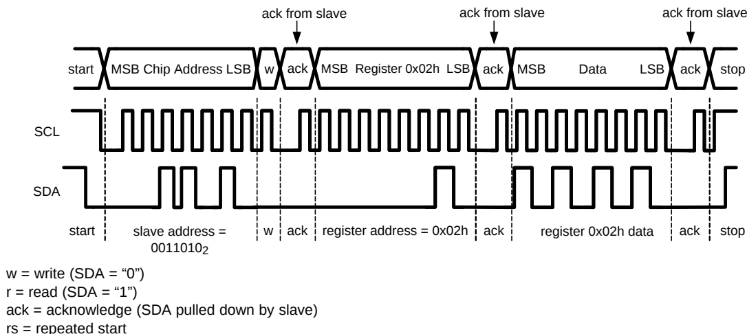
Figure 26. Example I²C Write Cycle
