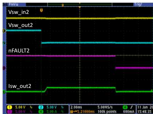
Figure 31. Power Switch2 Current Limit Operation
