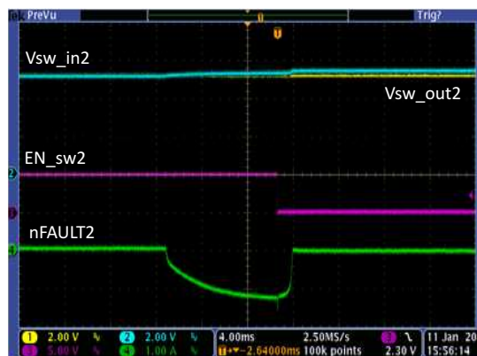
Figure 33. Power Switch2 Reverse Voltage Protection Response
