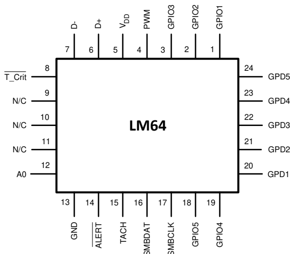
Figure 4-1. 24-pin WQFN Package
