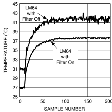
Figure 6-7. Digital Filter Response in an Intel Pentium 4 processor System
