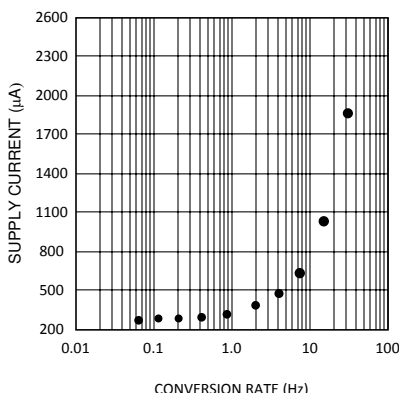
Figure 6-1. Supply Current vs Conversion Rate
