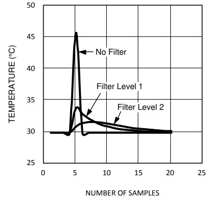
Figure 6-6. Impulse Response of the Digital Filter
