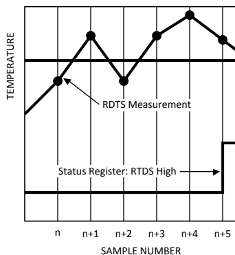
Figure 6-8. Fault Queue Temperature Response Diagram
