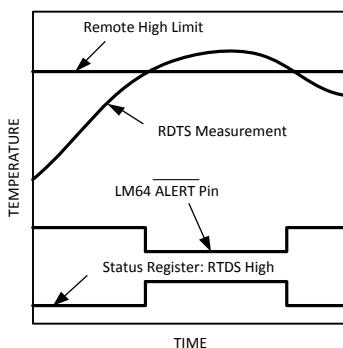
Figure 6-2. \overline{\text{ALERT}} Output as Temperature Comparator Response Diagram
