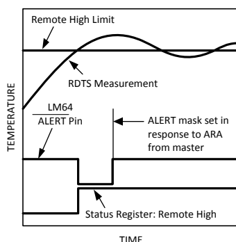
Figure 6-4. \overline{\text{ALERT}} Output as an SMBus ALERT Temperature Response Diagram
