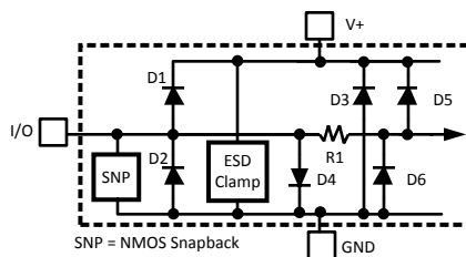
Figure 5-2. ESD Protection Input Structure
