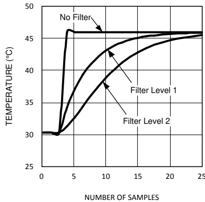
Figure 6-5. Step Response of the Digital Filter
