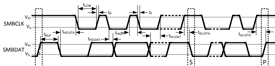
Figure 5-1. SMBus Timing Diagram for SMBCLK and SMBDAT Signals
