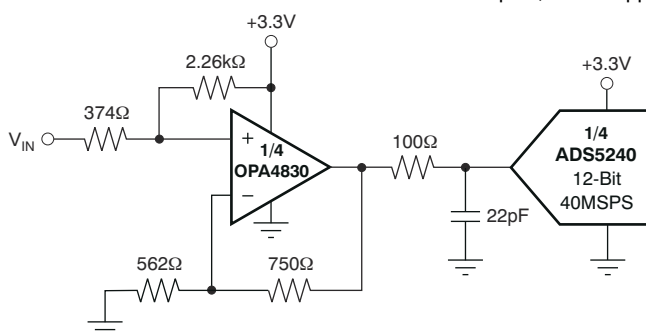
DC-Coupled, 3.3V ADC Driver
