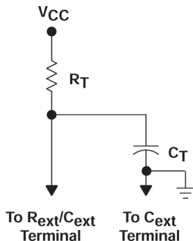
Figure 7-1. Timing-Component Connections
