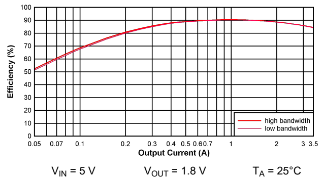
Figure 5-2. Efficiency BUCK1
