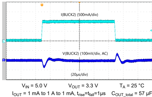
Figure 5-5. BUCK2 Load-step response - Low Bandwidth, forced PWM
