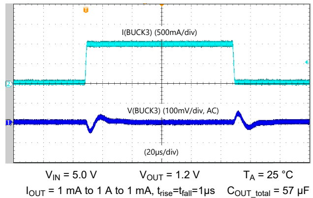
Figure 5-6. BUCK3 Load-step response - Low Bandwidth, forced PWM
