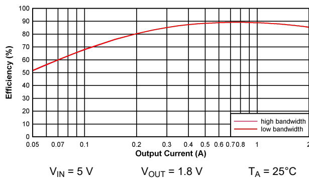
Figure 5-3. Efficiency BUCK23
