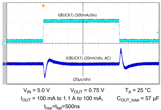
Figure 5-4. BUCK1 Load-step response - High Bandwidth, forced PWM
