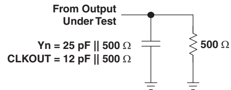
Figure 7. Test Load Circuit
