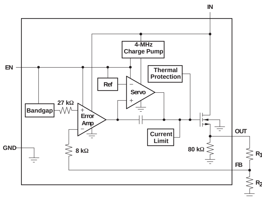
Figure 3. Adjustable-Voltage Version
