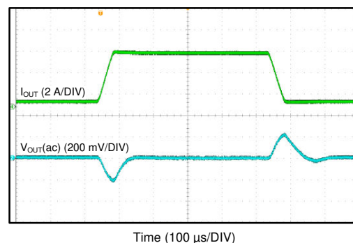
Figure 7-5. DCM Mode
