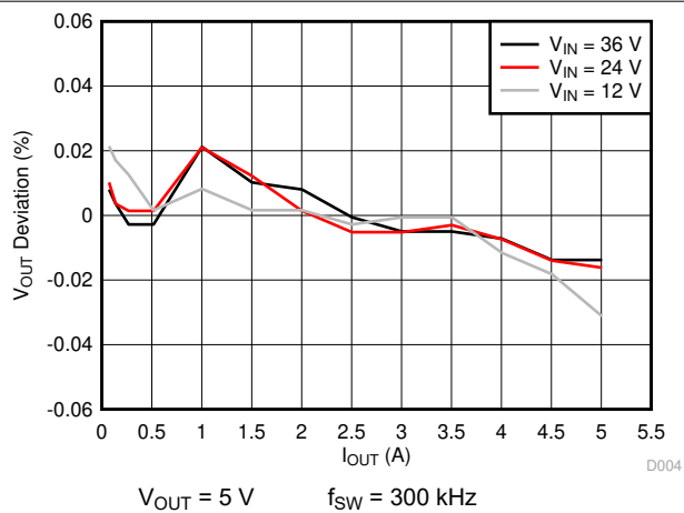
Figure 5-5. Load Regulation
