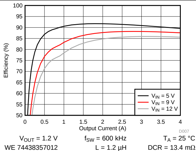
Figure 5. Efficiency for 1.2 V Output
