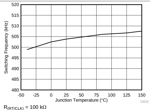
Figure 22. Switching Frequency vs Junction Temperature (500 kHz)
