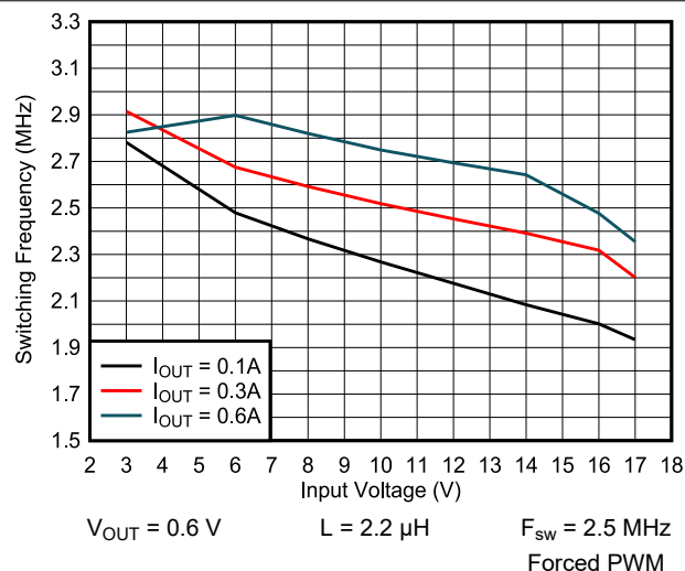
Figure 9-53. Switching Frequency vs Input Voltage
