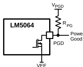
Figure 13. Power Good Output
