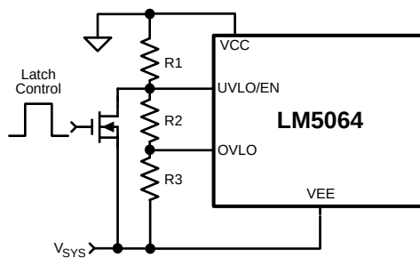
Figure 3. Latched Fault Restart Control
