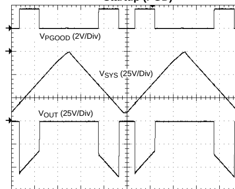
Startup (PGD)
