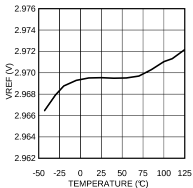
Reference Voltage
