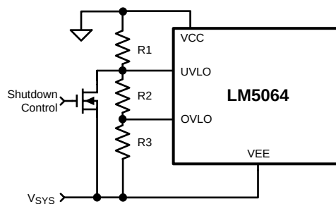
Figure 5. Shutdown Control
