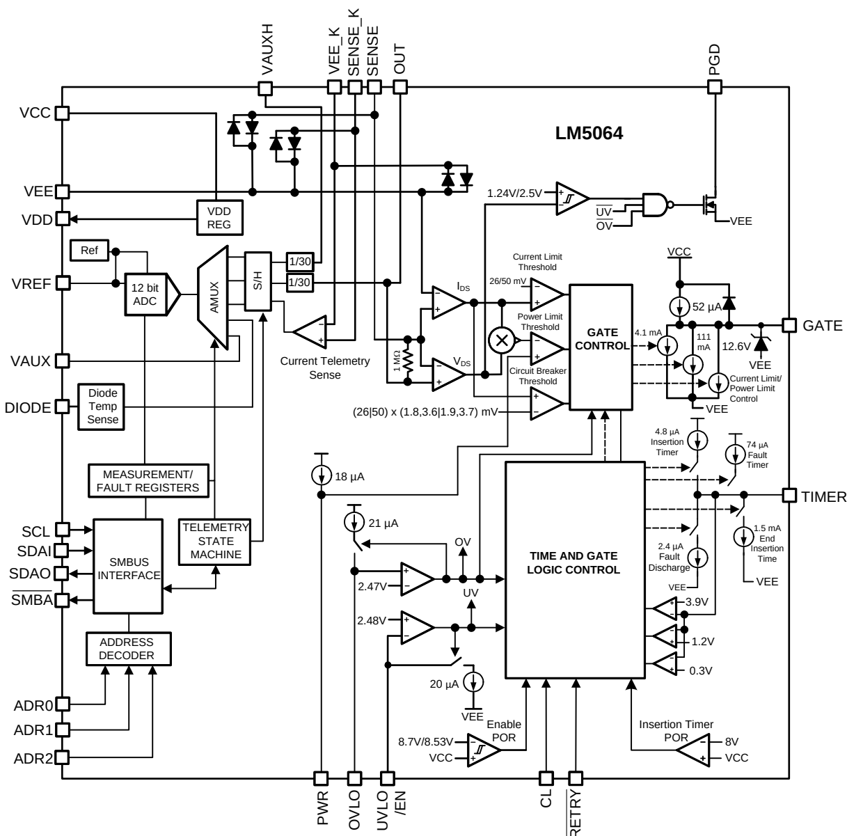
Figure 1. Block Diagram
