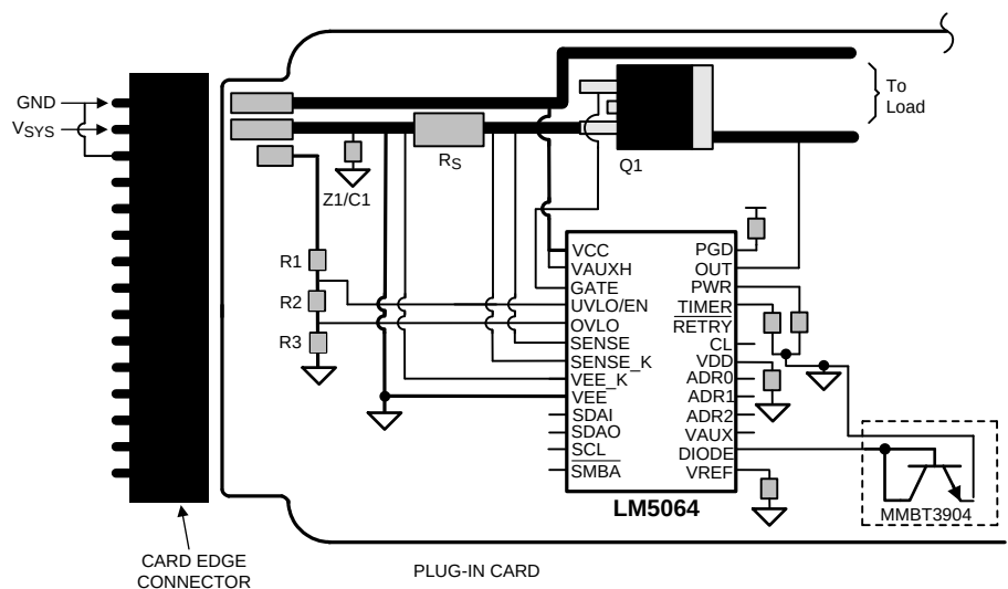
Figure 18. Recommended Board Connector Design
