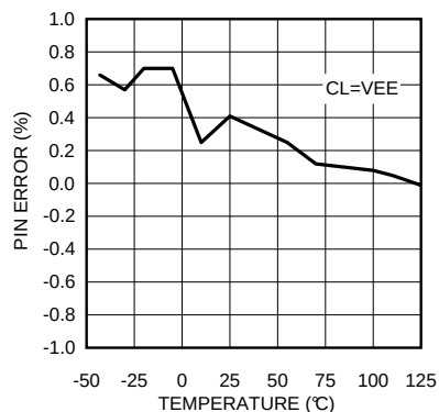
PIN Measurement Accuracy (SENSE_K-VEE_K = 50 mV)
