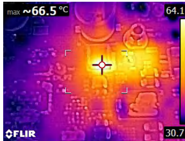
Figure 7-24. Thermal Image at 25^\circ\text{C} Ambient
