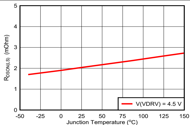
Figure 5-2. Low-Side FET R DS(ON)
