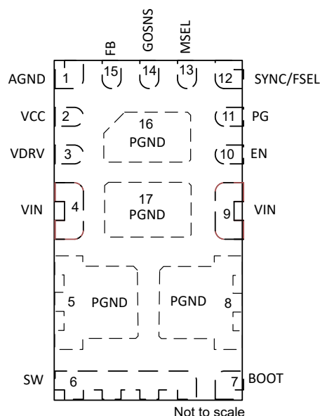
Figure 4-2. 17-Pin WQFN-FCRLF RYS Package (Top View)
