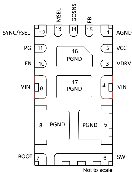
Figure 4-1. 17-Pin WQFN-FCRLF RYS Package (Bottom View)
