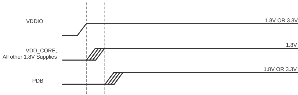
Figure 42. Power-Up Sequencing
