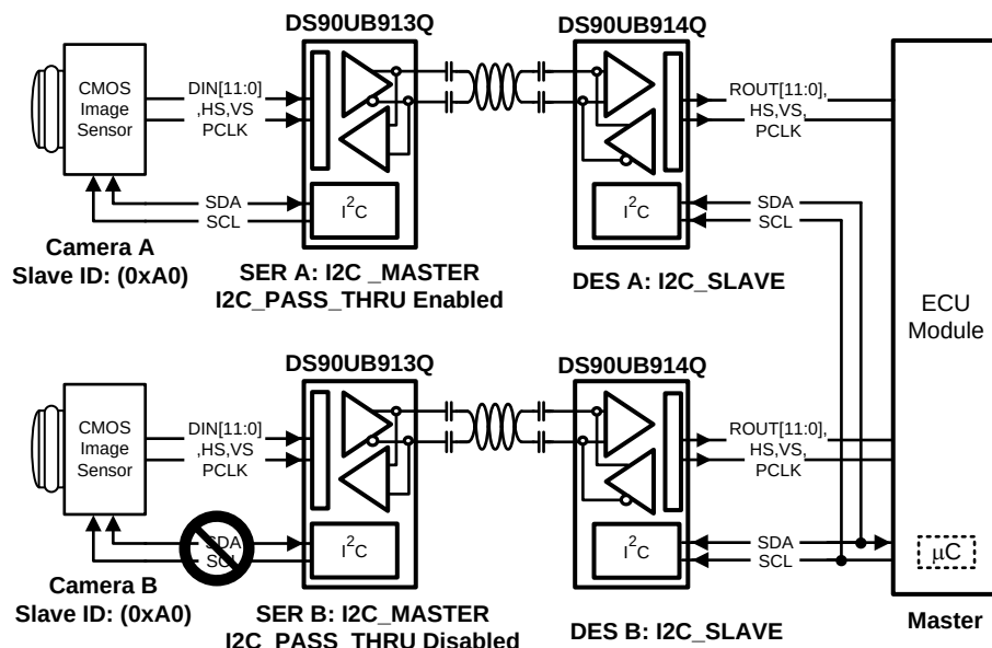
Figure 30. I²C Pass-Through
