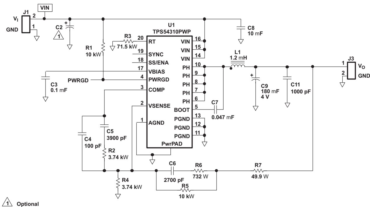
Figure 10. TPS54310 Schematic
