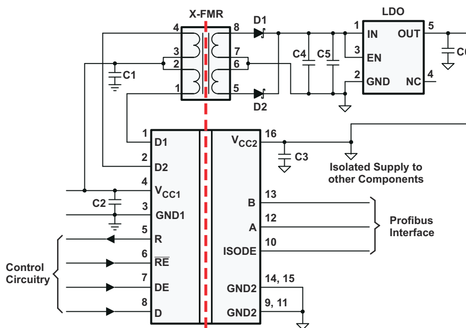
Figure 9-2. Typical Application
