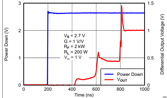
Figure 20. Turnon Time
