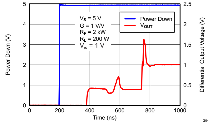
Figure 53. Turnon Time
