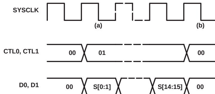
Figure 18. Status Transfer Timing
