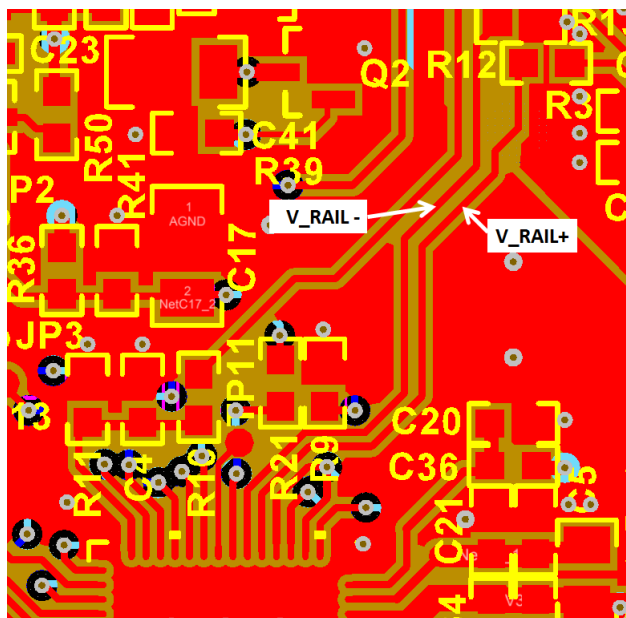
Figure 19. Balanced Differential Signal Layout
