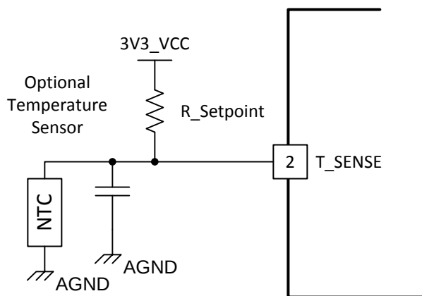
Figure 5. NTC Application
