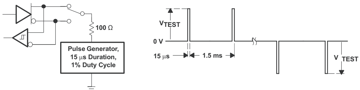
Figure 9-16. Test Circuit and Waveforms, Transient Overvoltage Test
