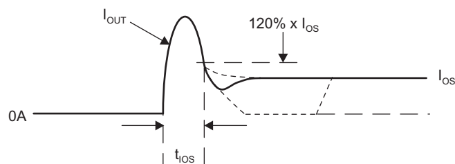
Figure 2. Response Time to Short Circuit Waveform
