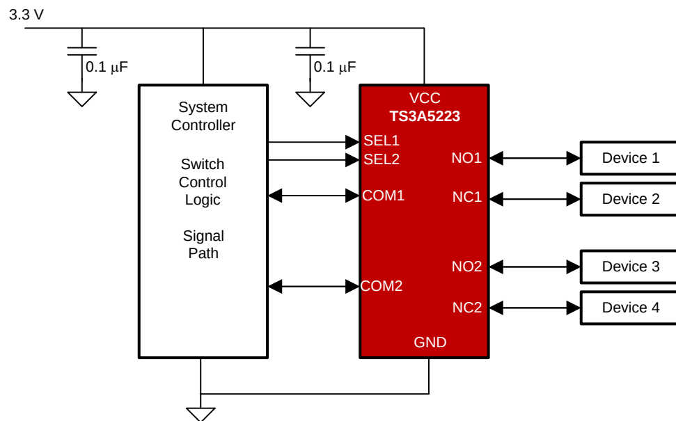
Figure 13. Typical Application
