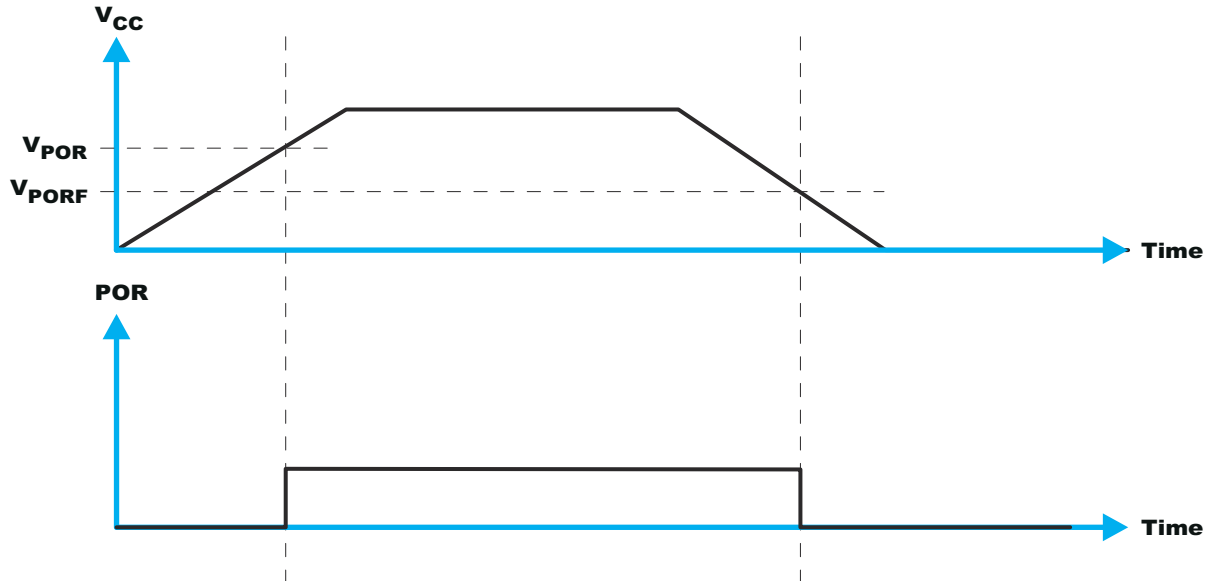
Figure 9-9. V_{POR}
