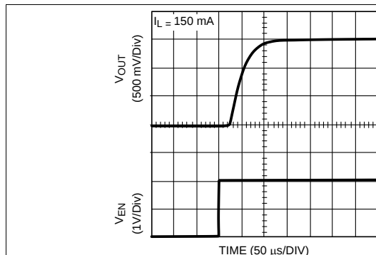
Figure 15. Enable Start-Up Time
