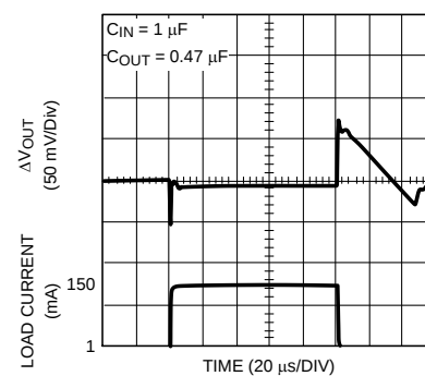
Figure 16. Load Transient
