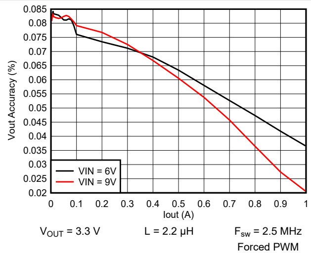
Figure 9-19. Output Voltage vs Output Current
