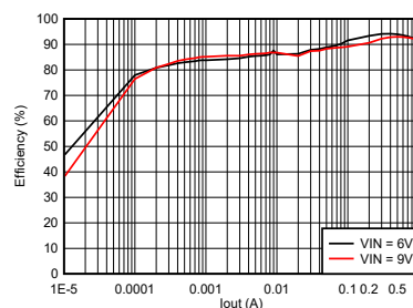
Efficiency Versus Output Current V_{\text{OUT}} = 3.3 \text{ V} at 2.5-MHz Auto PFM/PWM
