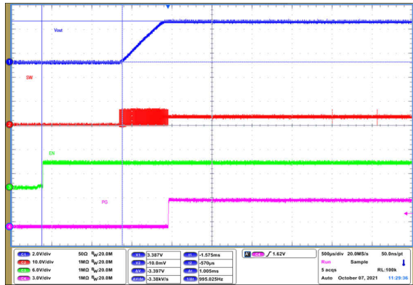
Figure 9-62. Start-Up Timing
