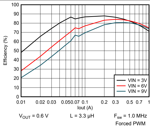
Figure 9-57. Efficiency vs Output Current
