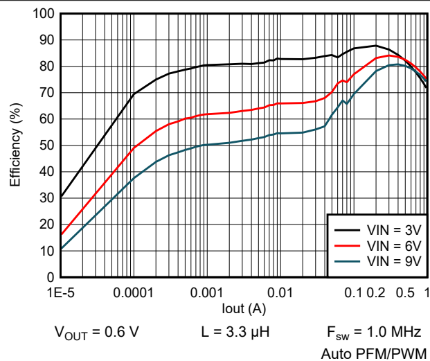
Figure 9-56. Efficiency vs Output Current
