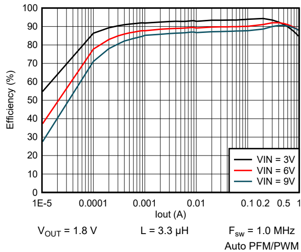
Figure 9-32. Efficiency vs Output Current
