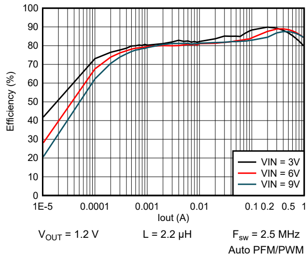
Figure 9-38. Efficiency vs Output Current
