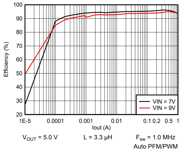
Figure 9-8. Efficiency vs Output Current
