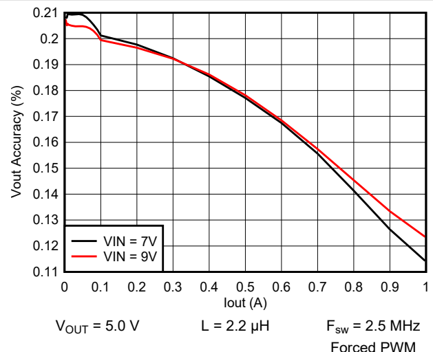
Figure 9-7. Output Voltage vs Output Current
