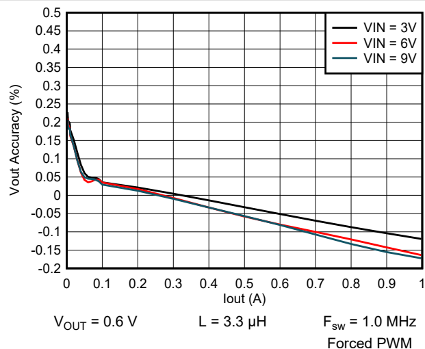
Figure 9-61. Output Voltage vs Output Current
