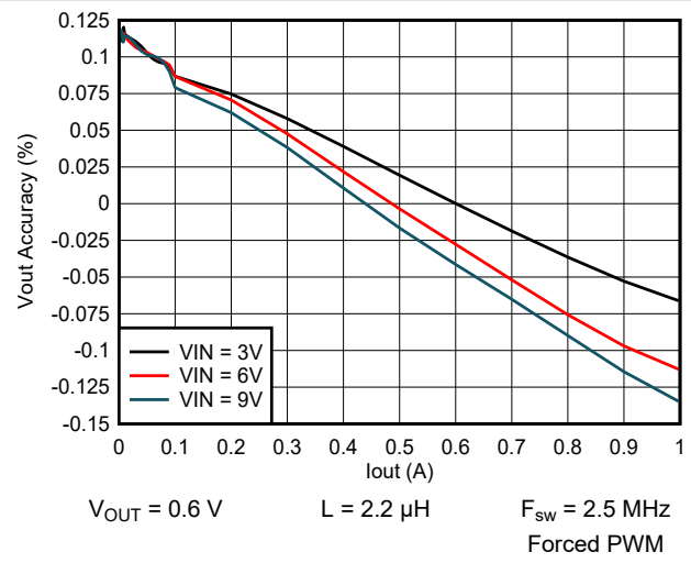
Figure 9-55. Output Voltage vs Output Current
