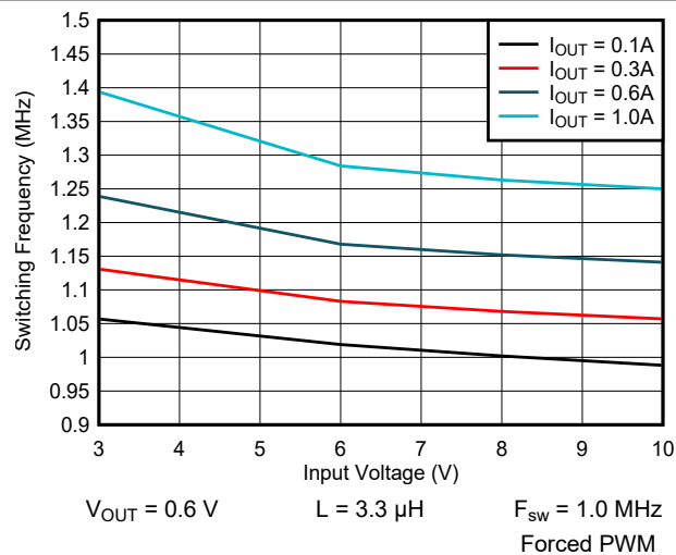
Figure 9-59. Switching Frequency vs Input Voltage
