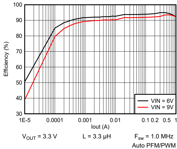
Figure 9-20. Efficiency vs Output Current
