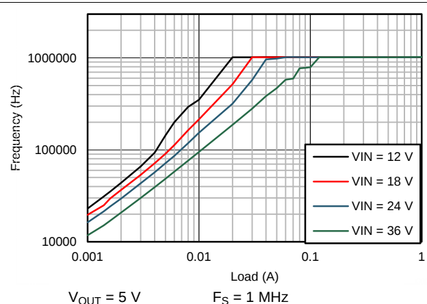
Figure 94. Switching Frequency vs I_{OUT} in PFM Operation
