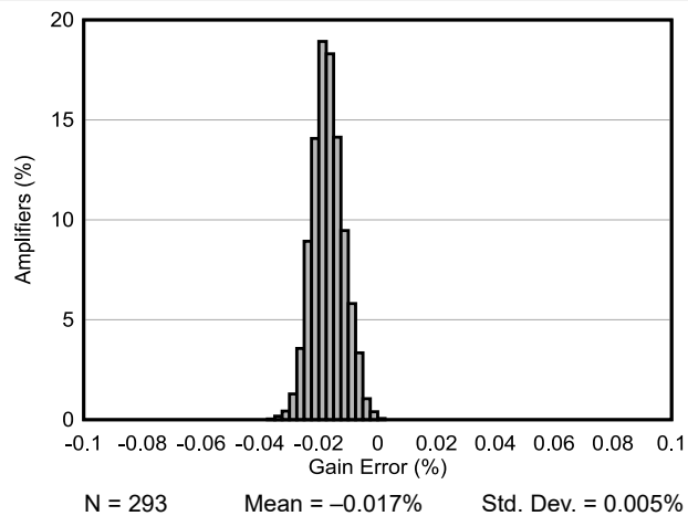
Figure 7-11. Typical Gain Error Distribution at G = 0.2 V/V
