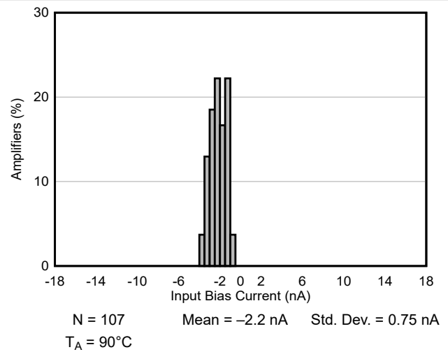
Figure 7-8. Typical Distribution of Input Bias Current
