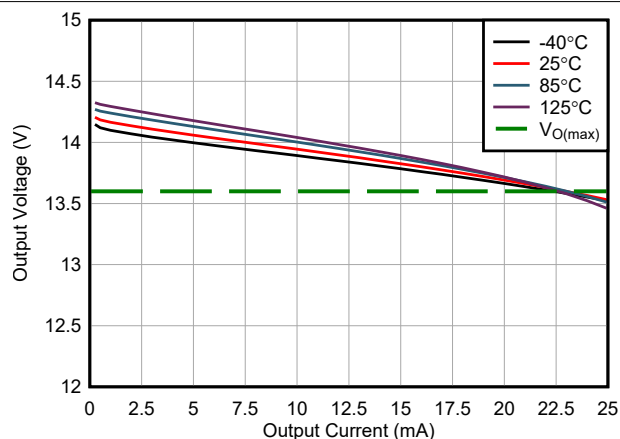
Figure 7-38. Positive Output Voltage Swing vs Output Current
