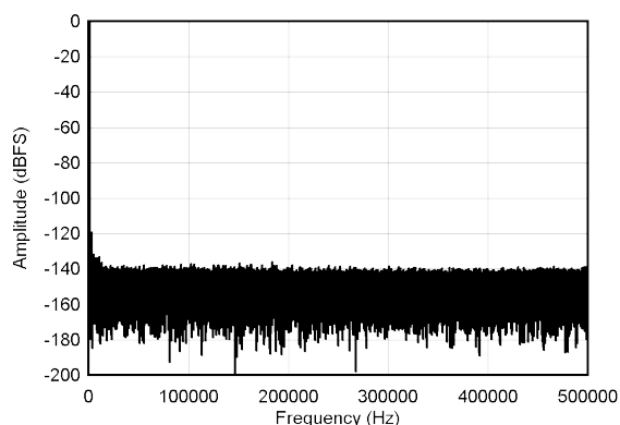
Figure 9-7. Noise Performance FFT Plots for G = 0.2\text{ V/V}
