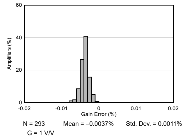
Figure 7-12. Typical Gain Error Distribution at G = 1 V/V
