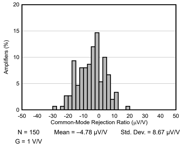
Figure 7-9. Typical CMRR Distribution at G = 1 V/V
