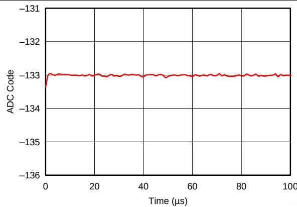
Figure 31. Reference Droop
