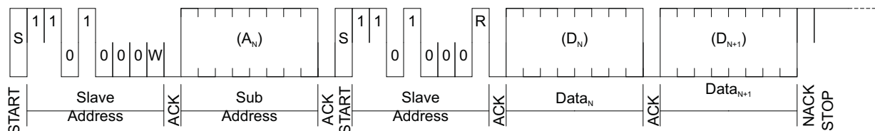
Figure 7. I²C Read Mode
