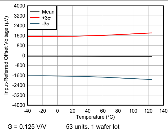
Figure 7-19. Offset Voltage (RTI) vs Temperature
