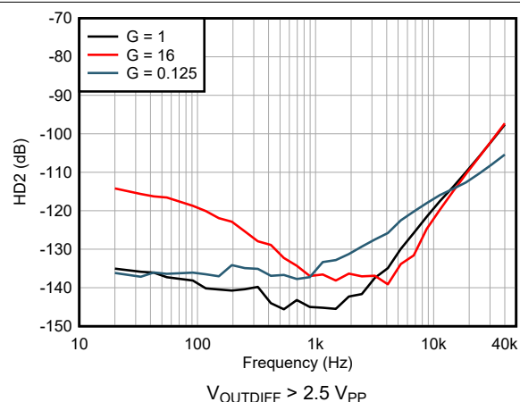
Figure 7-56. 2nd Harmonic Distortion vs Frequency
