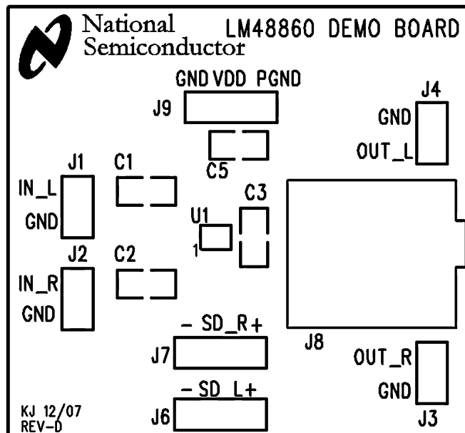
Figure 38. Top Silkscreen
