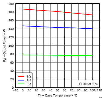
Figure 7. Output Power vs Temperature
