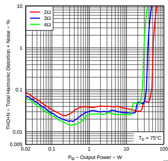
Figure 9. Total Harmonic Distortion + Noise vs Output Power
