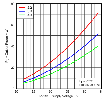
Figure 10. Output Power vs Supply Voltage
