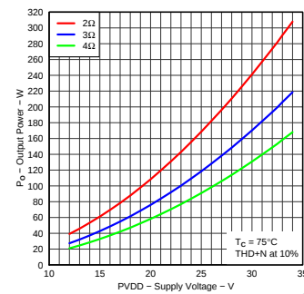
Figure 12. Output Power vs Supply Voltage
