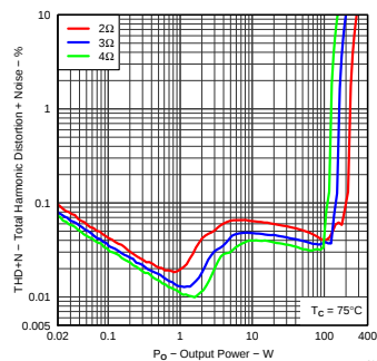
Figure 11. Total Harmonic Distortion + Noise vs Output Power
