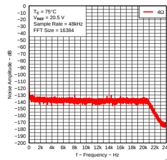
Figure 8. Noise Amplitude vs Frequency
