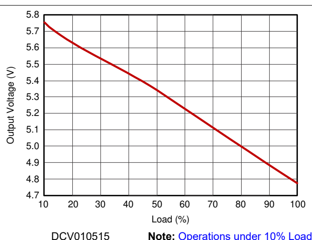
DCV010515 Note: Operations under 10% Load Figure 9-4. Load Regulation
