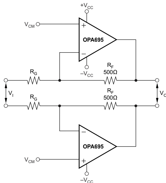
Figure 7-9. Inverting Input Differential I/O Amplifier
