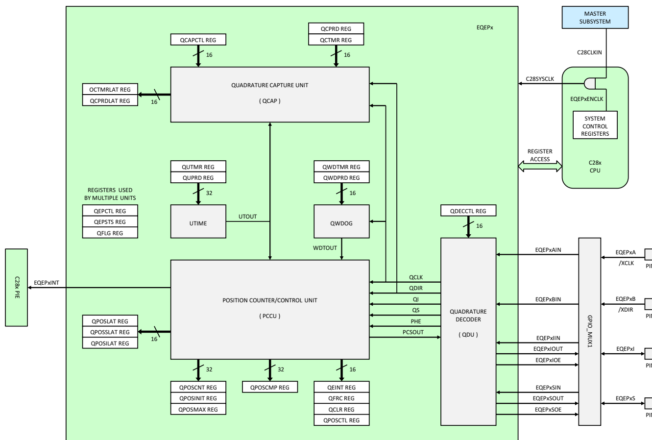
Figure 7-47. eQEP
