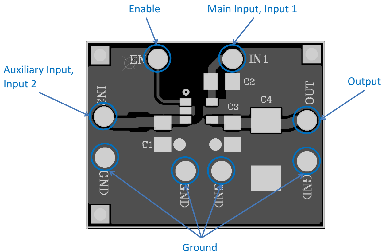
Figure 21. Enable, Input, Output, and Ground Pins
