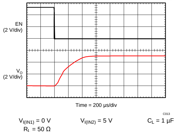
Figure 16. Propagation Delay and Rise Time With 1- \mu F Load, IN2 Turnon
