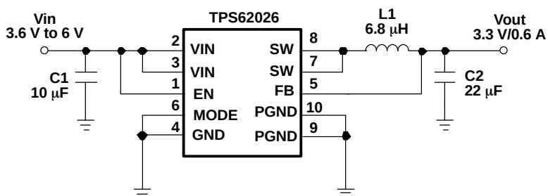
Figure 20. TPS62026 Fixed 3.3 V Output Using 6.8 µH inductor
