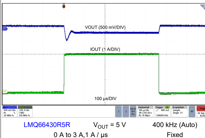
Figure 9-8. Load Transient
