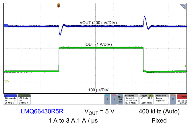
Figure 9-9. Load Transient
