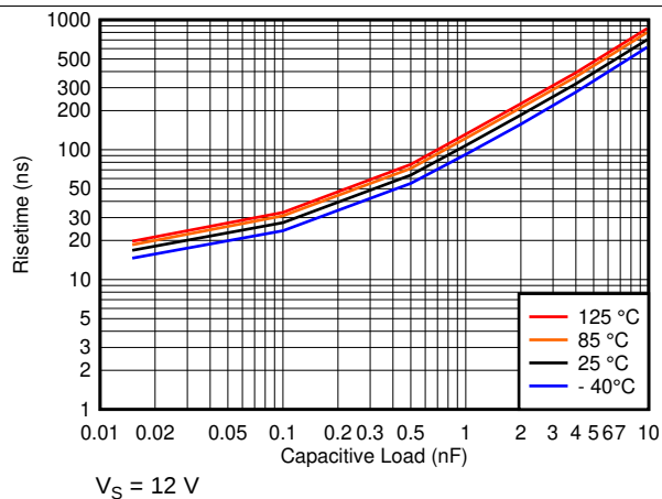
Figure 55. t_{\text{RISE}} vs. Capacitive Load at 12V
