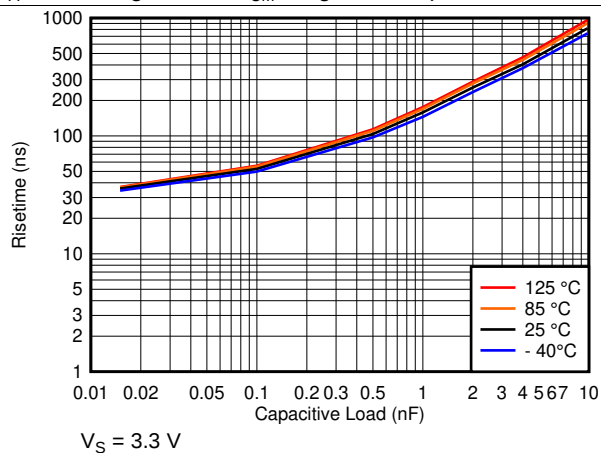
Figure 51. t_{\text{RISE}} vs. Capacitive Load at 3.3V
