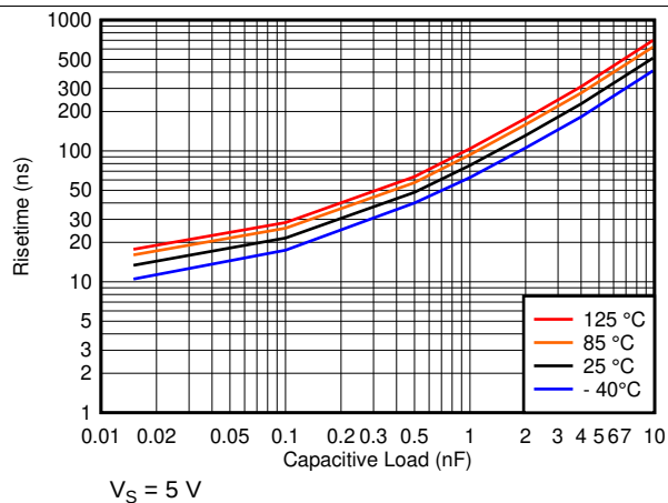
Figure 53. t_{\text{RISE}} vs. Capacitive Load at 5V
