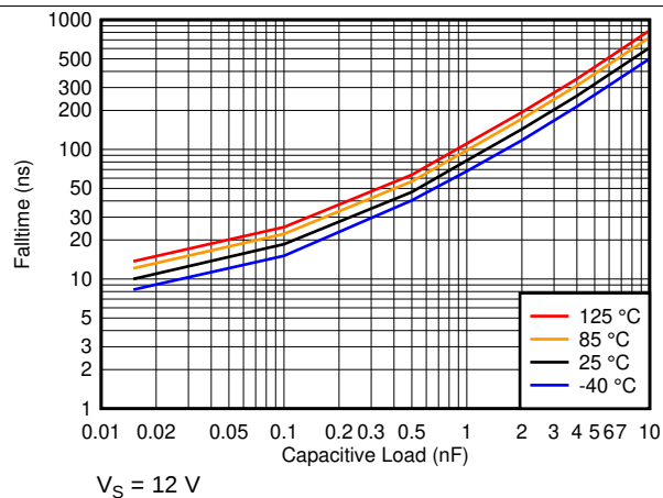
Figure 56. t_{\text{FALL}} vs. Capacitive Load at 12V
