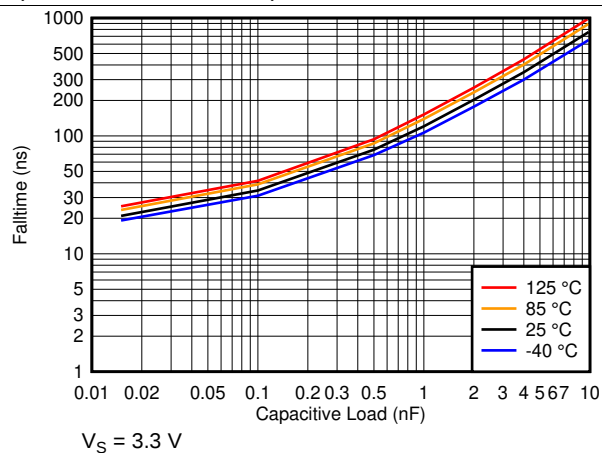
Figure 52. t_{\text{FALL}} vs. Capacitive Load at 3.3V
