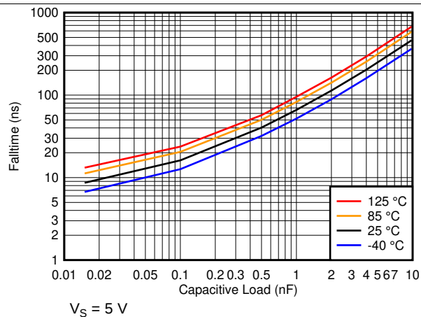
Figure 54. t_{\text{FALL}} vs. Capacitive Load at 5V
