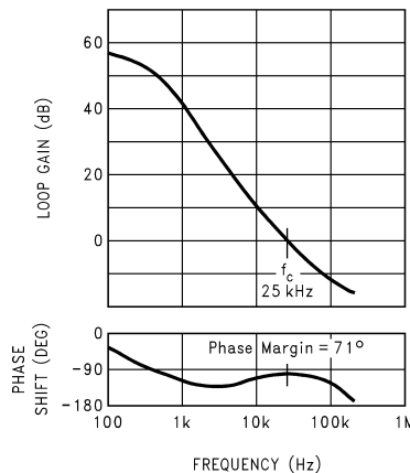
Figure 29. Measured Gain/Phase Plot for 3.3V/4A Application
