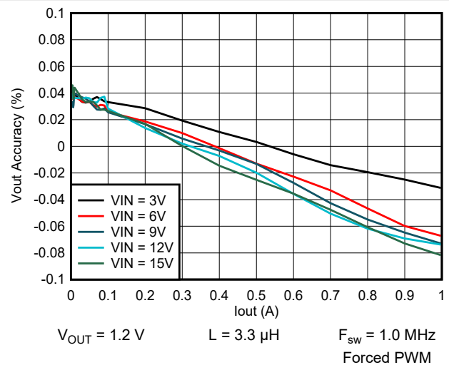
Figure 9-49. Output Voltage vs Output Current
