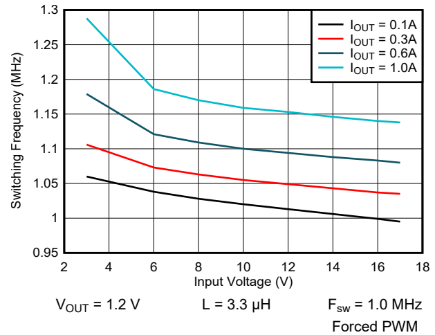
Figure 9-47. Switching Frequency vs Input Voltage
