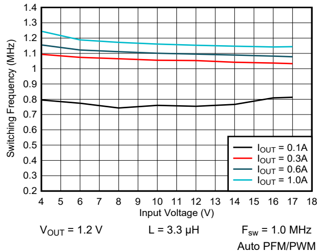
Figure 9-46. Switching Frequency vs Input Voltage
