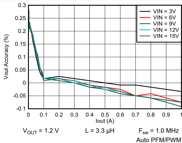
Figure 9-48. Output Voltage vs Output Current
